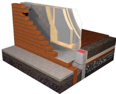
Cavity walls: QW in timber frame*
