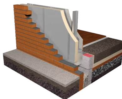
Cavity walls: QW in steel stud frame
