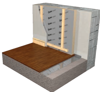
Solid walls: internal dry lining QW fixed by battens
